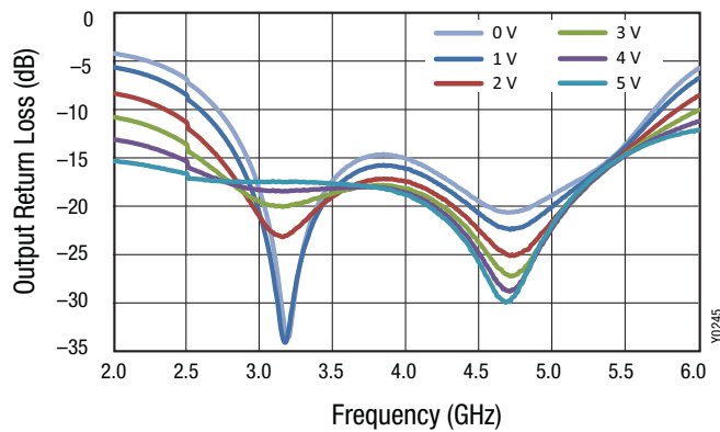
Figure 8. Output Return Loss vs Frequency Over Control Voltage
